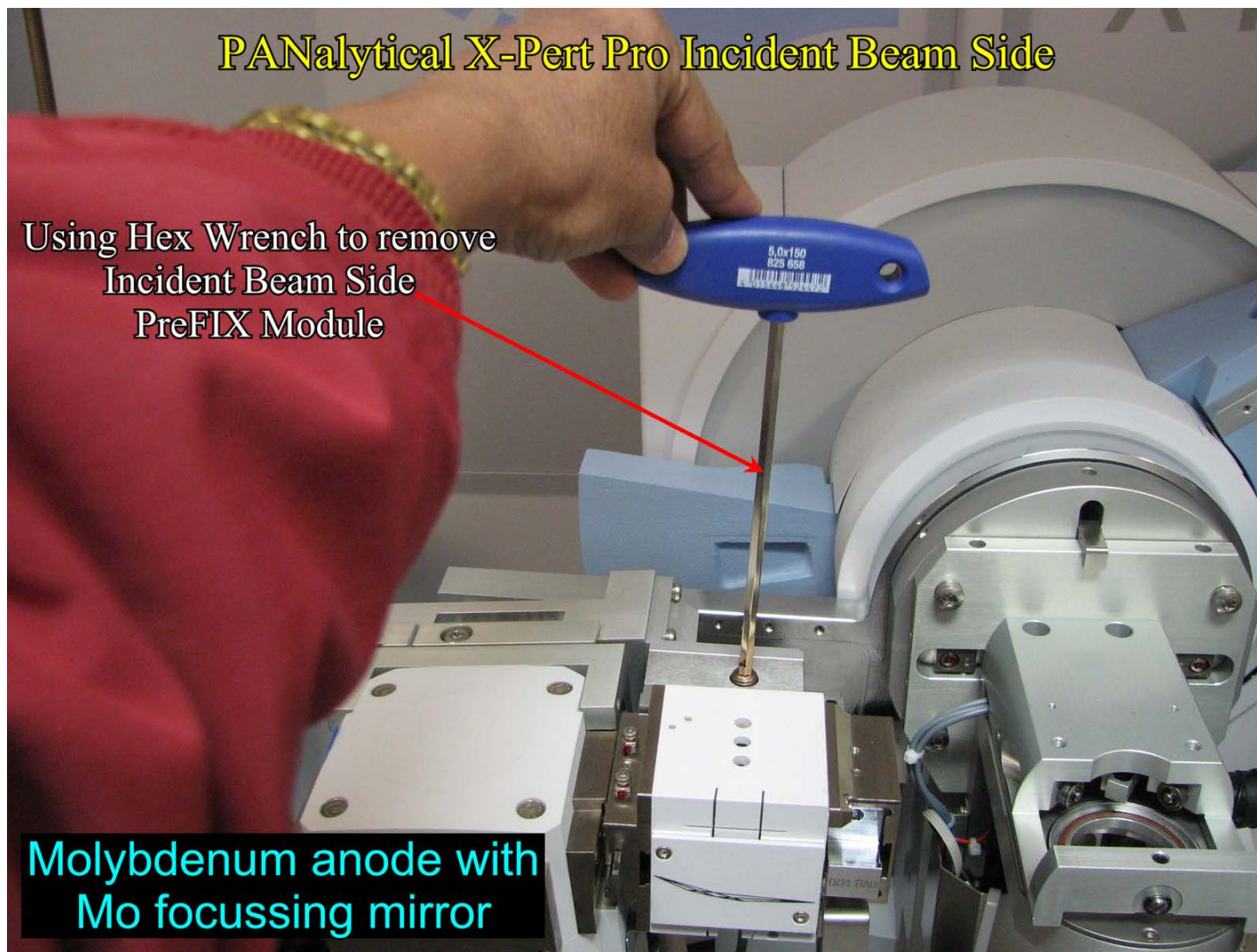
PANalytical X-Pert Pro Powder Instrument at FSU CSL 1011 using hex wrench to remove incident beam side Mo Mirror PreFIX module
